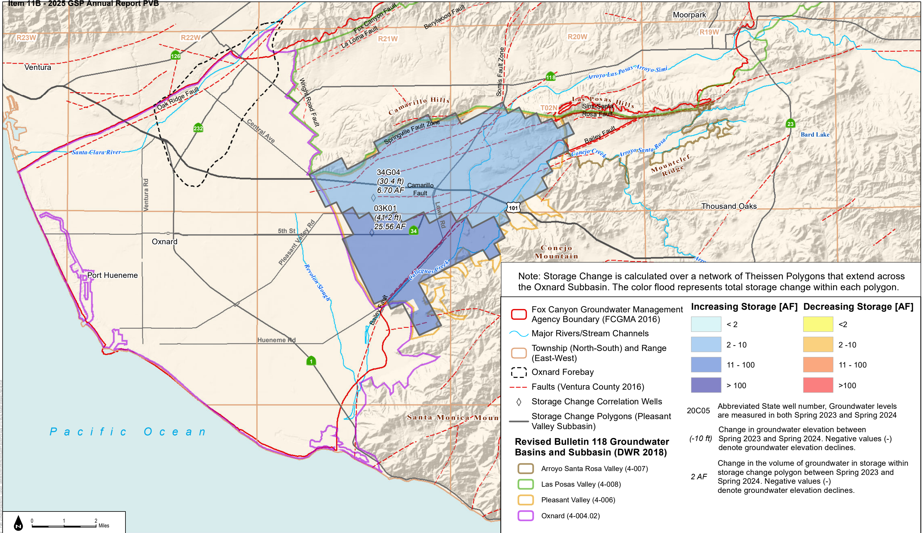
FIGURE 2-15 Change in Storage in the Mugu Aquifer: Spring 2023 to Spring 2024
