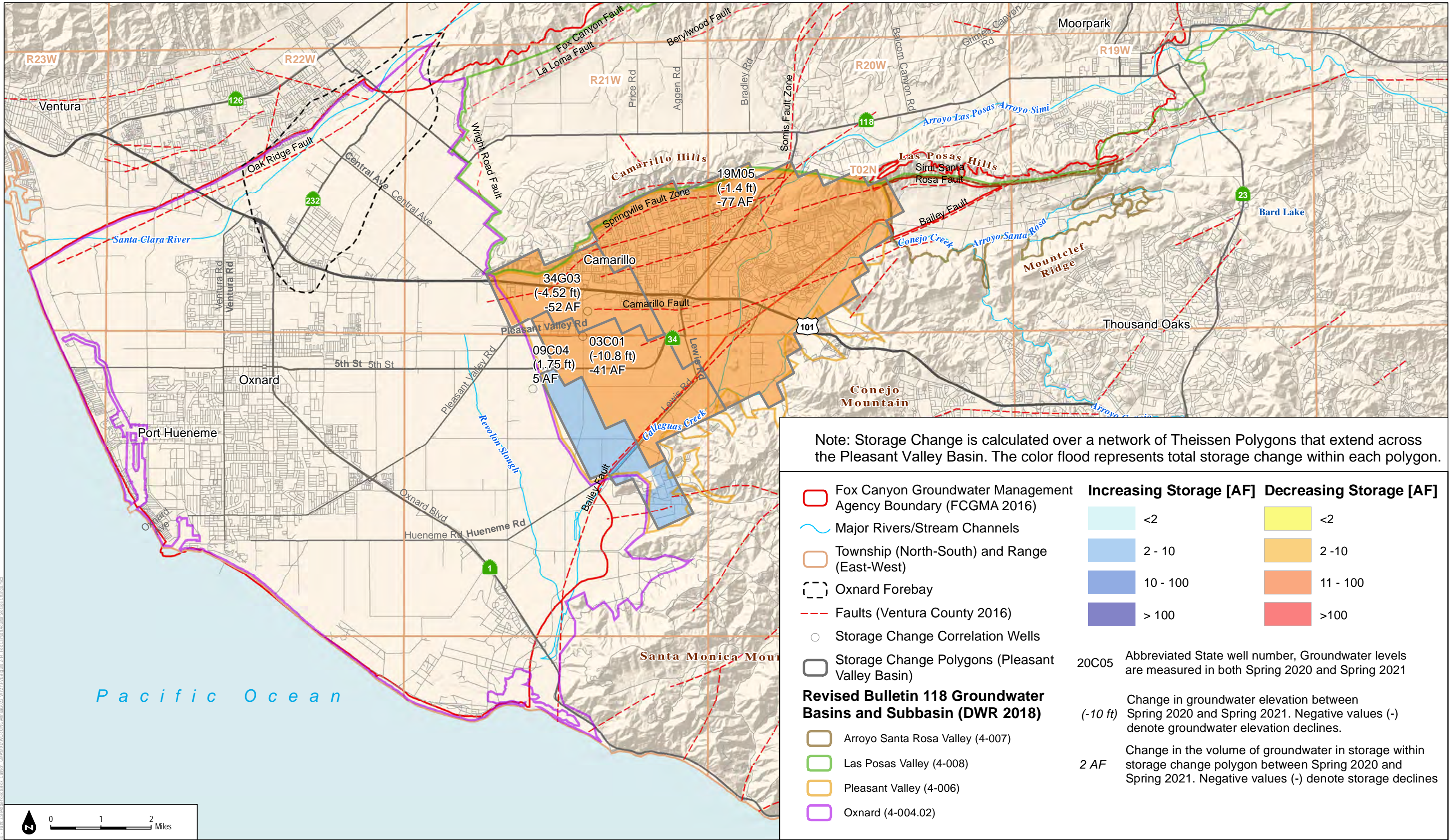
FIGURE 2-14 Change in Storage in the Fox Canyon Aquifer: Spring 2020 to Spring 2021
