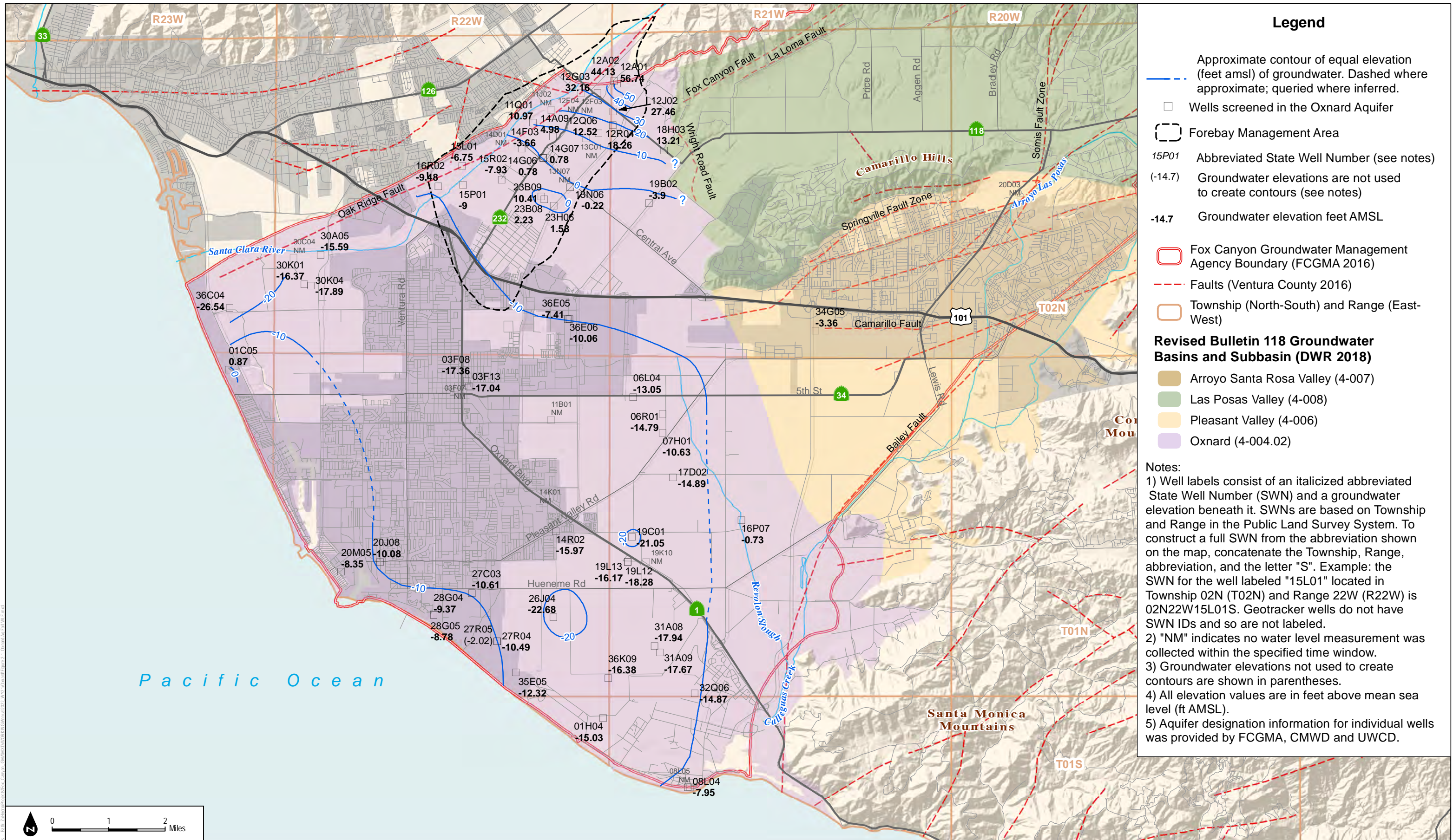
FIGURE 2-1 Groundwater Elevation Contours in the Oxnard Aquifer, October 2 to October 31, 2020
