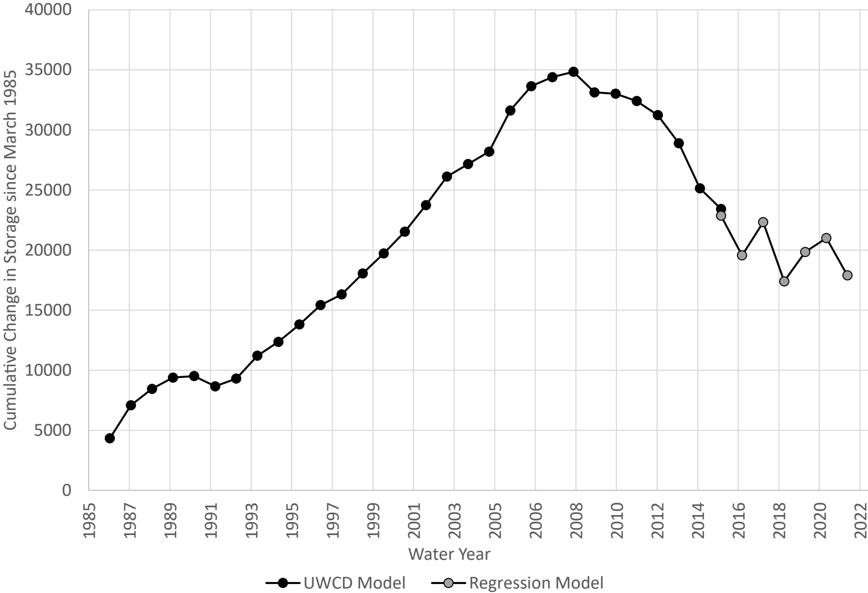
Validation of Linear Regression Model - Oxnard Aquifer
