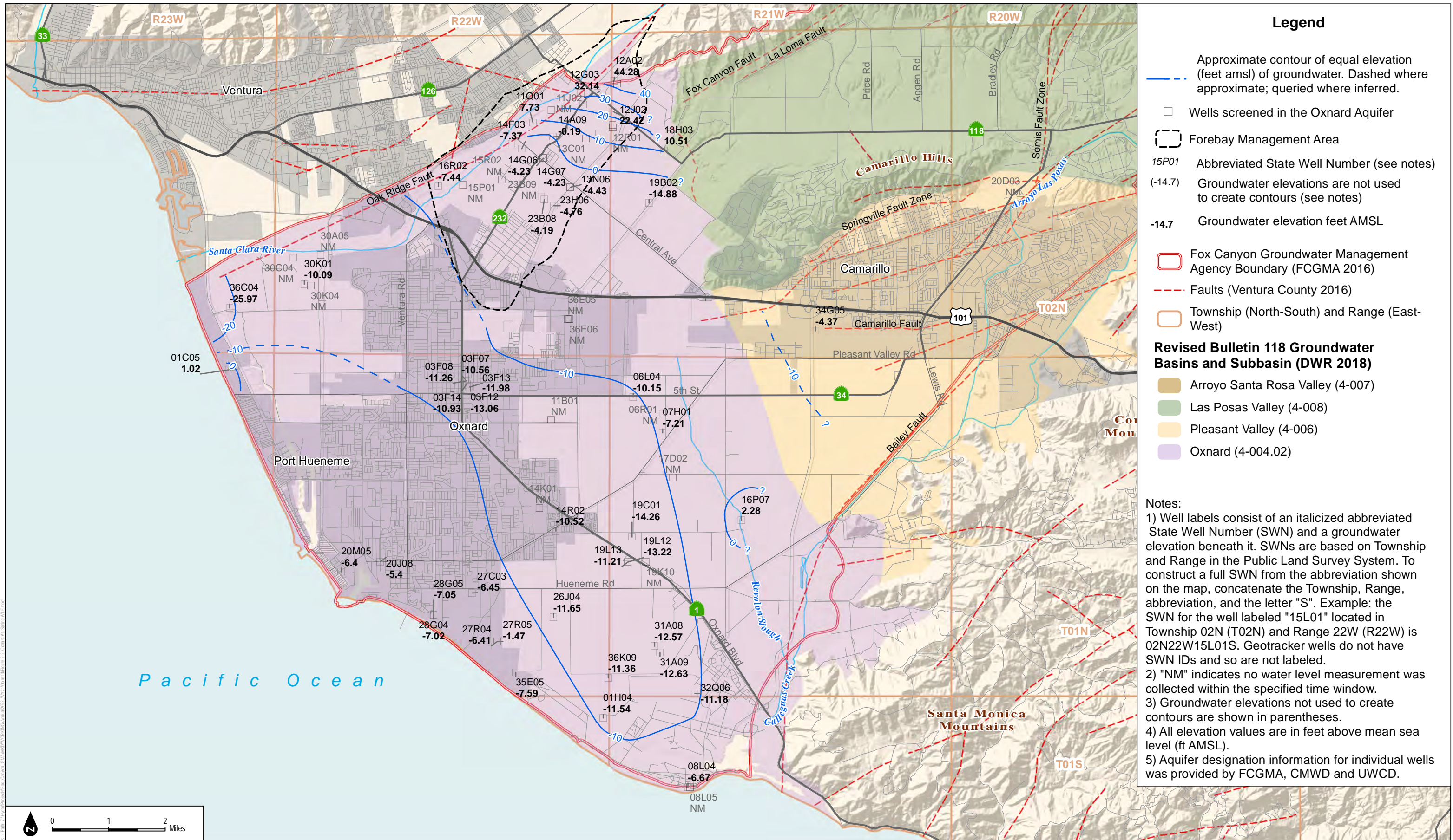
FIGURE 2-2 Groundwater Elevation Contours in the Oxnard Aquifer, March 2 to March 29, 2021
