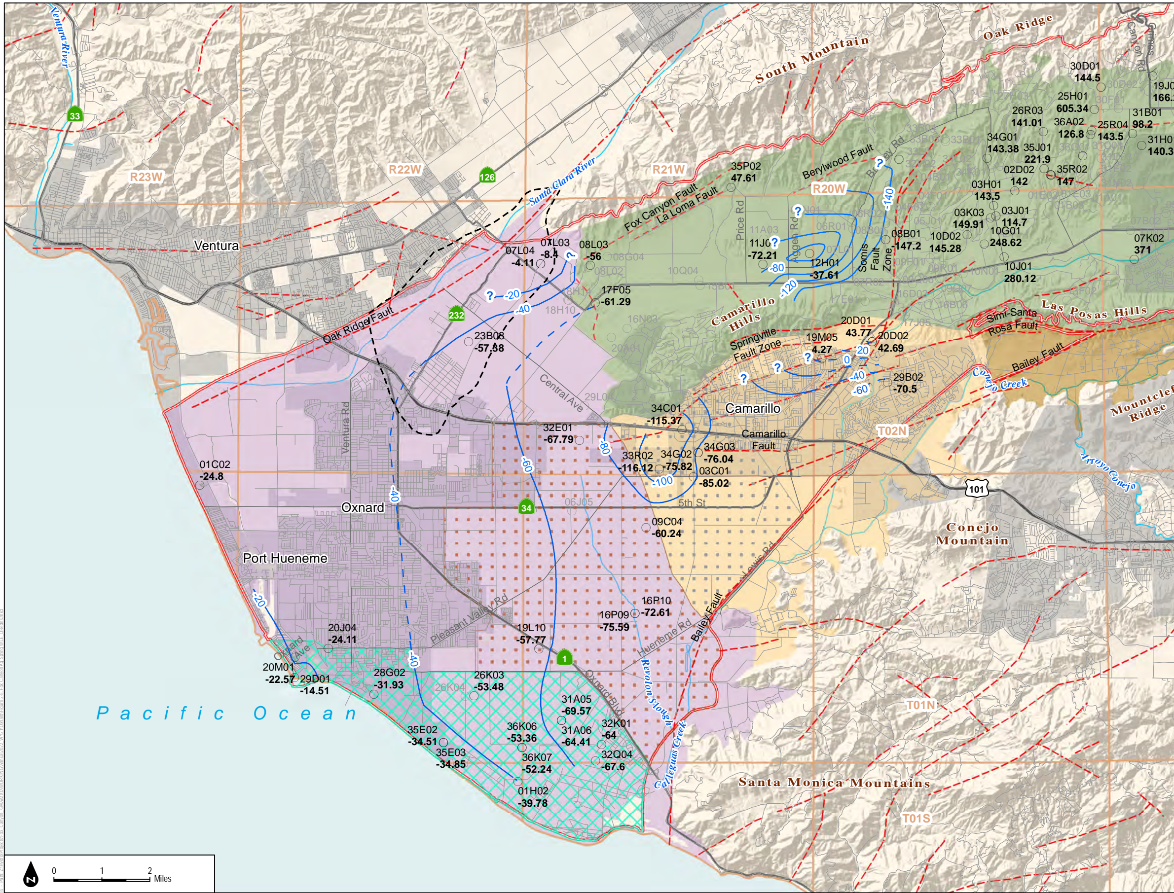
FIGURE 2-6 Groundwater Elevation Contours in the Fox Canyon Aquifer, March 2 to March 29, 2021
