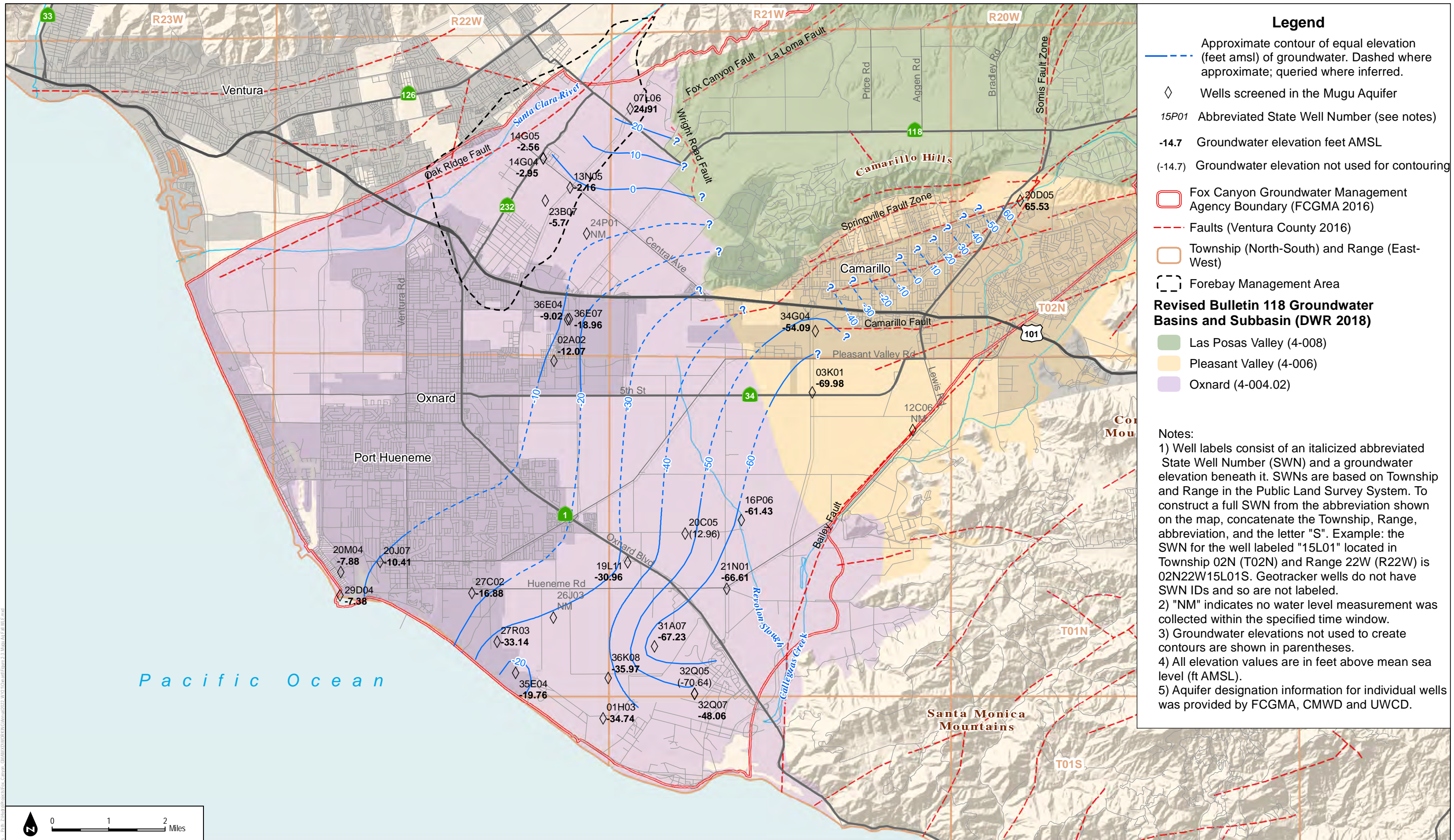
FIGURE 2-3 Groundwater Elevation Contours in the Mugu Aquifer, October 2 to October 31, 2020
