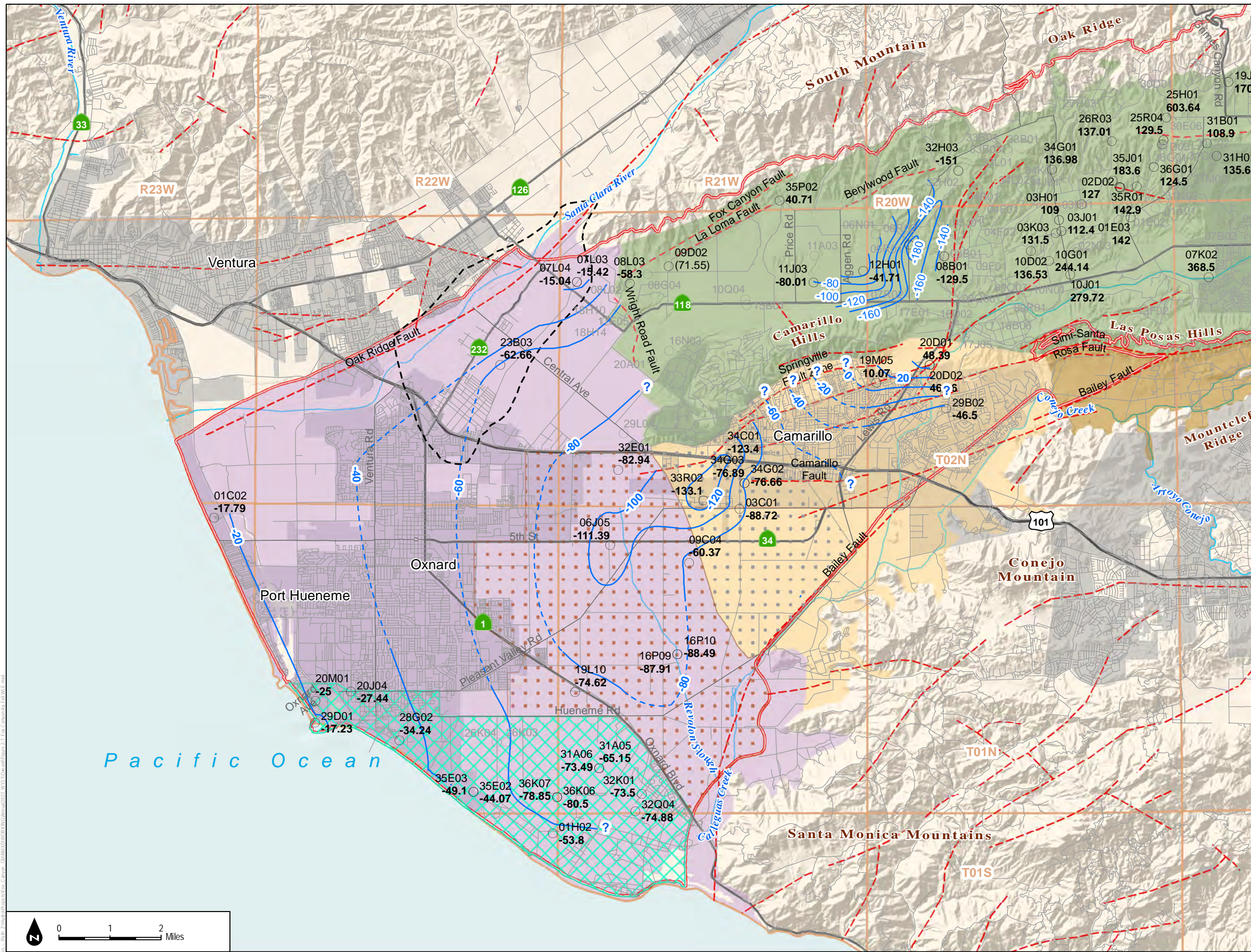
FIGURE 2-5 Groundwater Elevation Contours in the Fox Canyon Aquifer, October 2 to October 31, 2020
