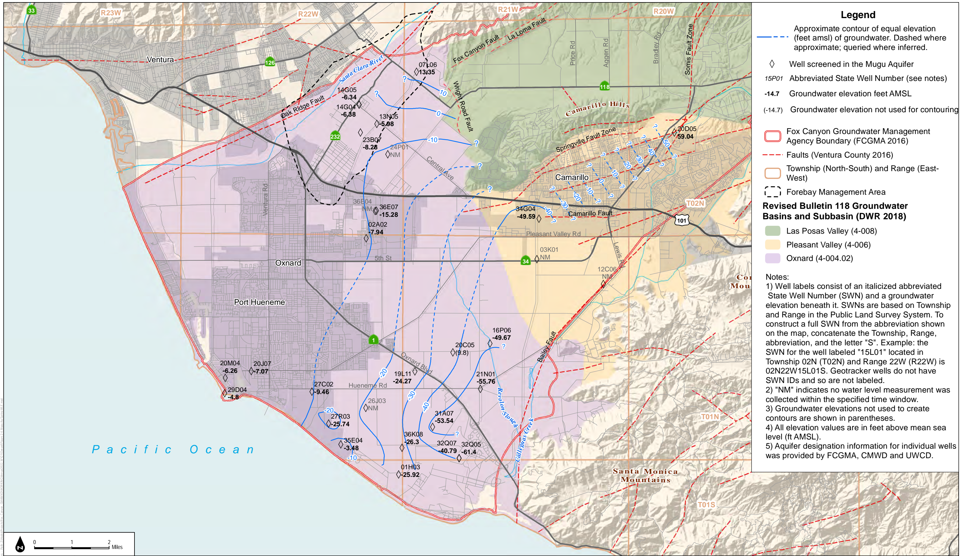
FIGURE 2-4 Groundwater Elevation Contours in the Mugu Aquifer, March 2 to March 29, 2021
