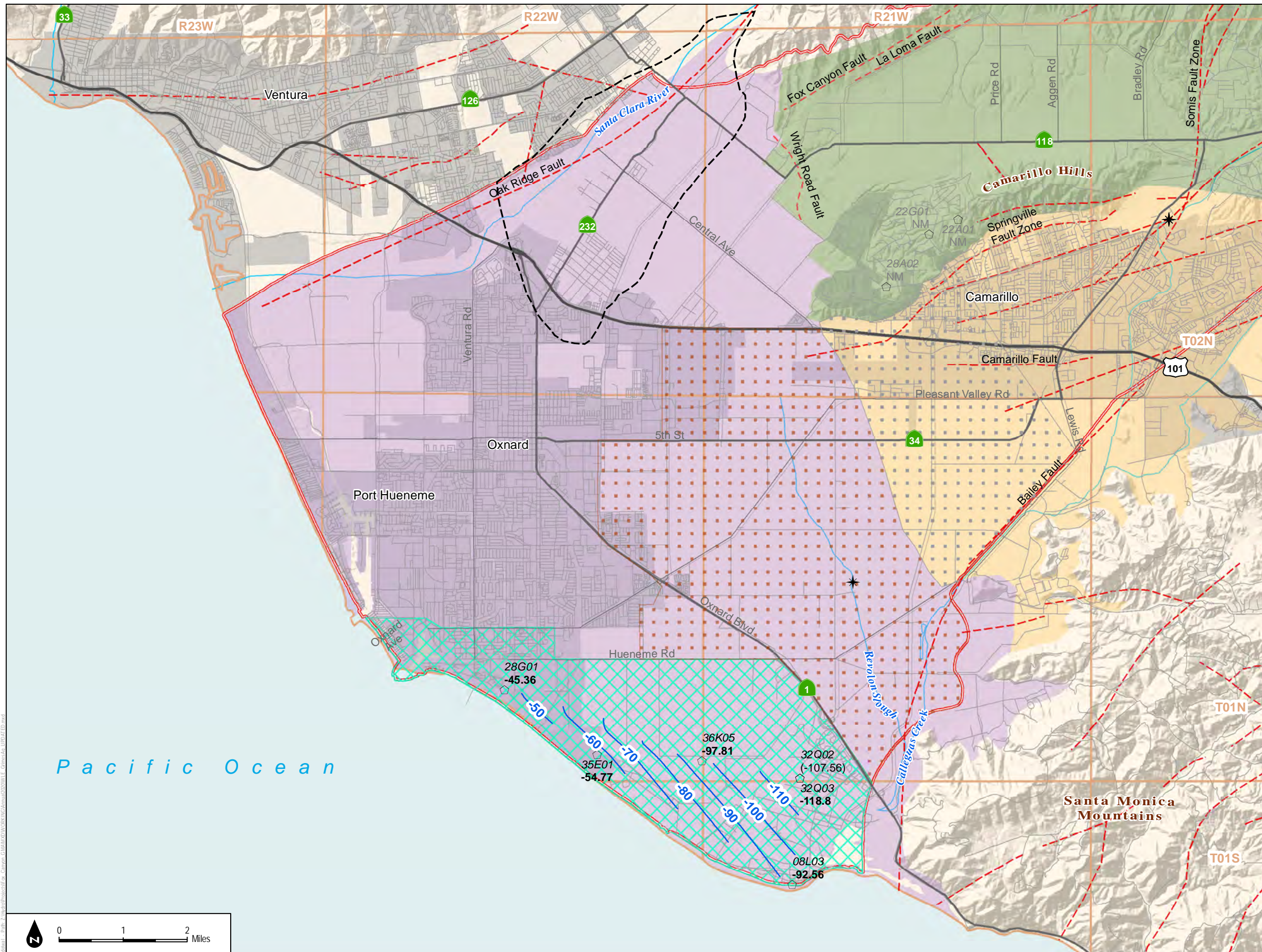
FIGURE 2-34 Groundwater Elevation Contours in the Grimes Canyon Aquifer, October 2-29, 2018
