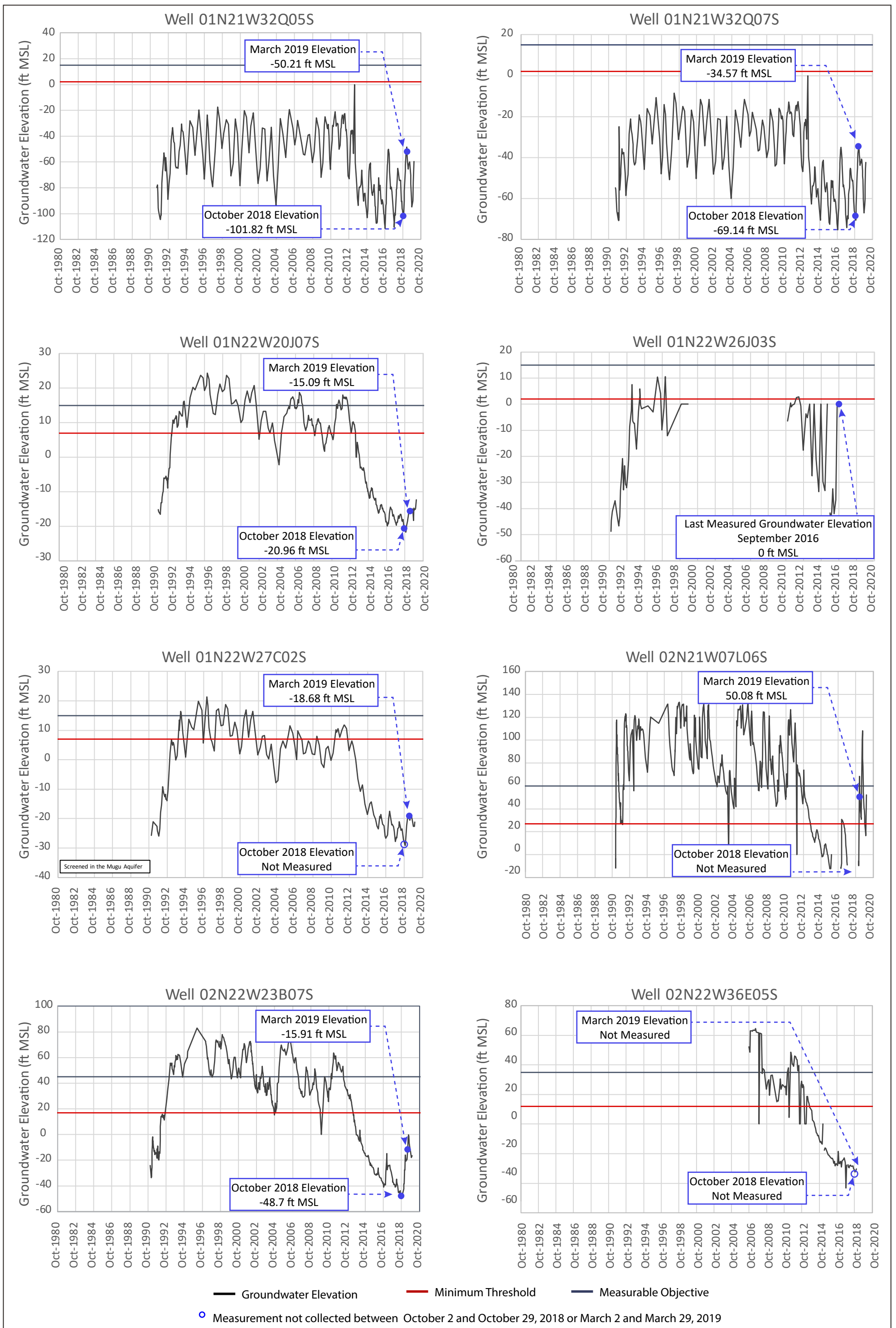
FIGURE 2-37 Groundwater Elevation Hydrographs for Representative Wells Screened in the Mugu Aquifer Oxnard Subbasin Groundwater Sustainability Plan 2020 Annual Report
