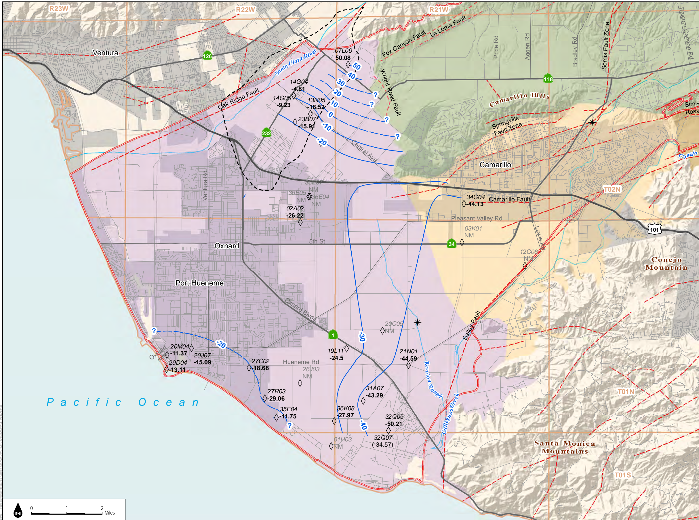
Groundwater Elevation Contours in the Mugu Aquifer, March 2-29, 2019
