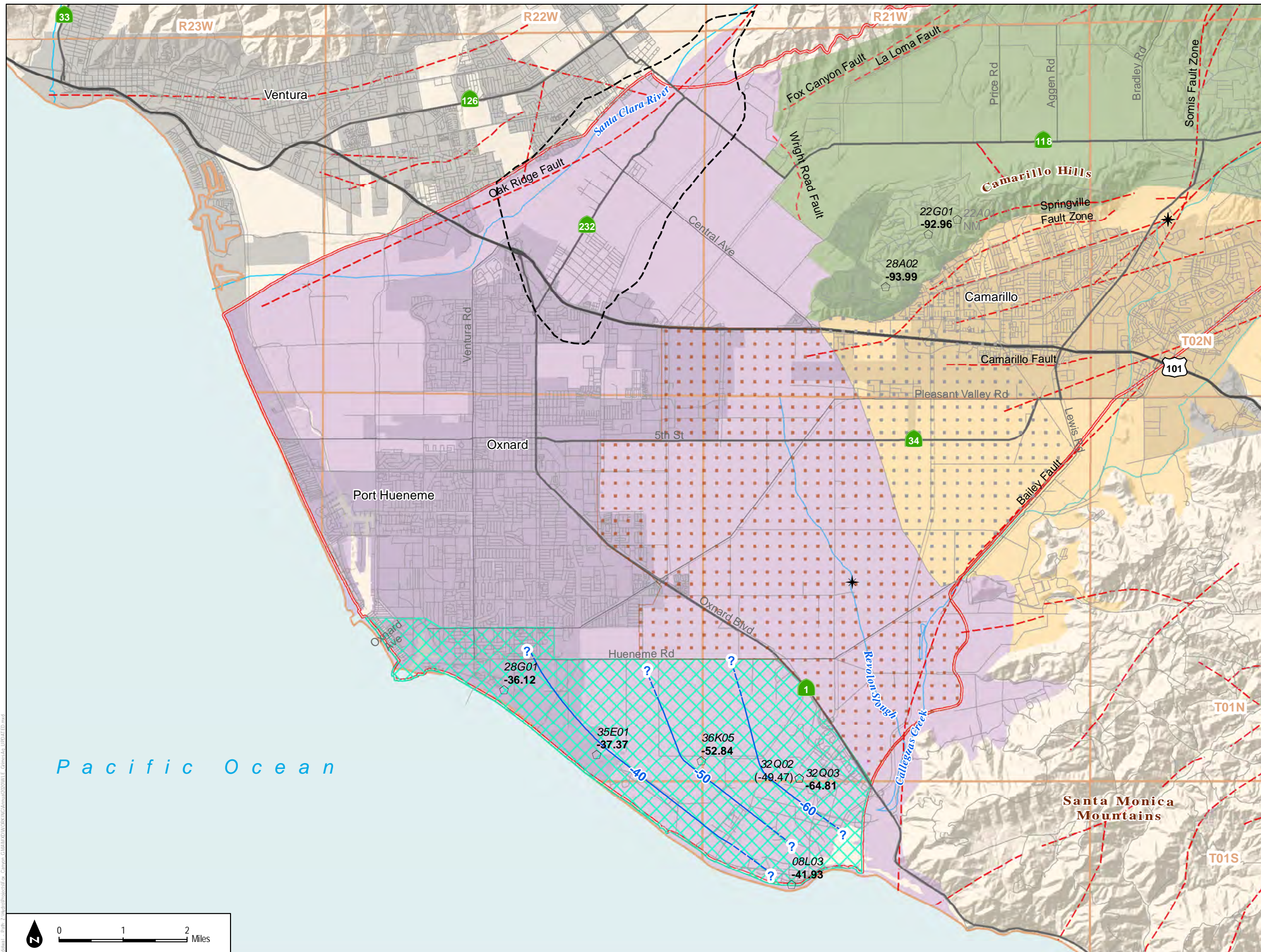
FIGURE 2-35 Groundwater Elevation Contours in the Grimes Canyon Aquifer, March 2-29, 2019
