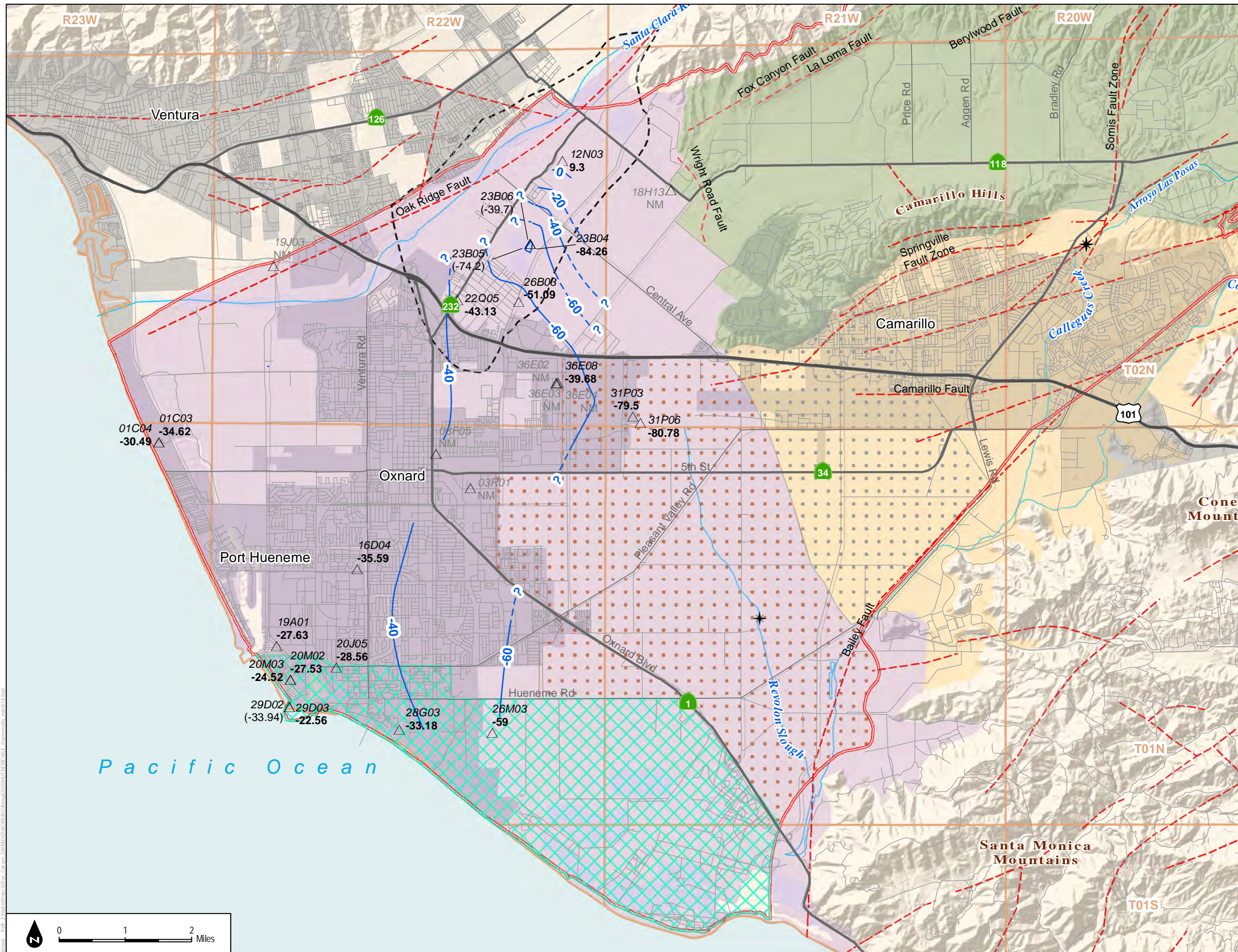
FIGURE 2-19 Groundwater Elevation Contours in the Hueneme Aquifer, March 2-29, 2018
