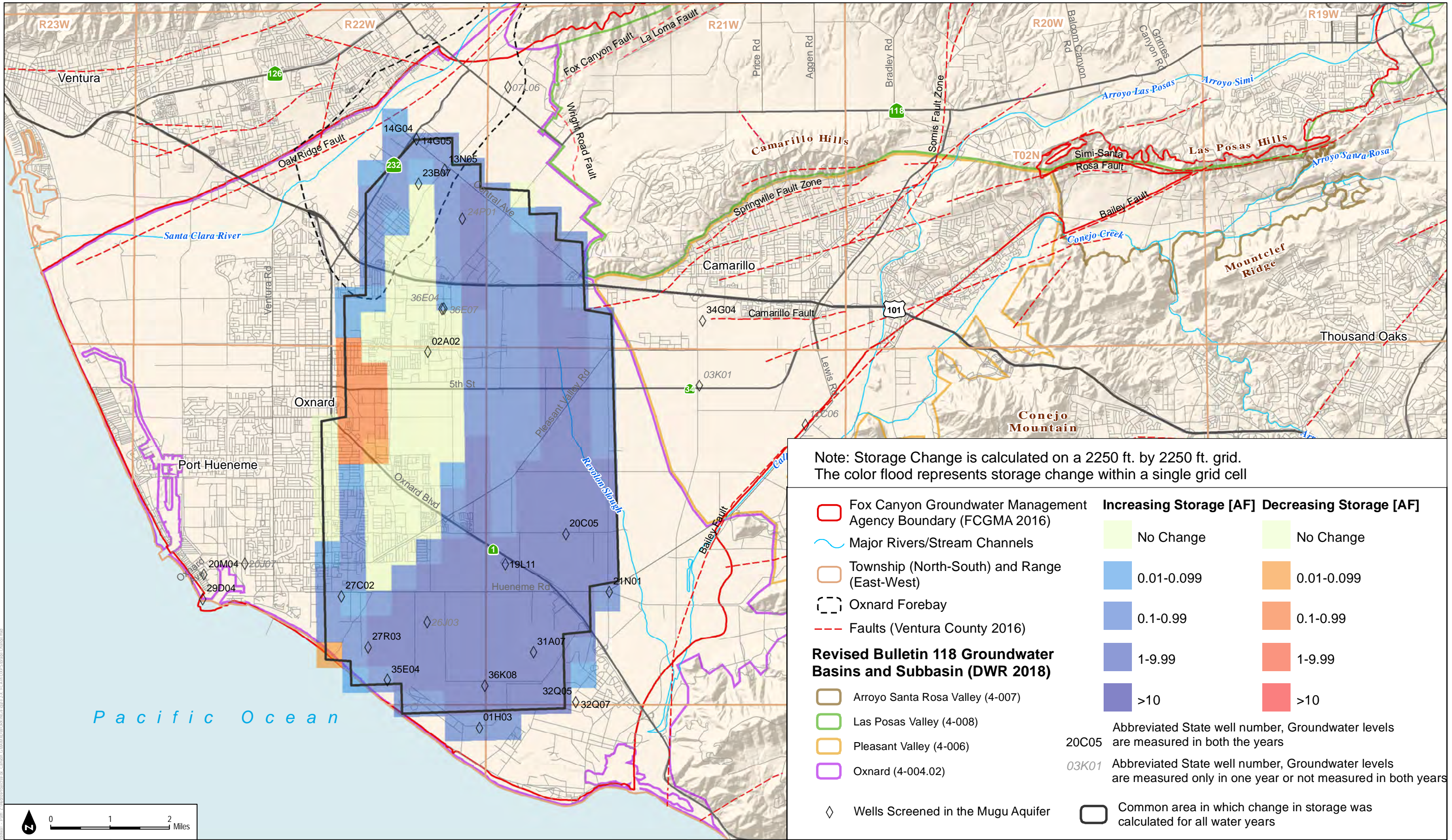
FIGURE 2-52 Change in Storage in the Mugu Aquifer: Spring 2016 to Spring 2017
