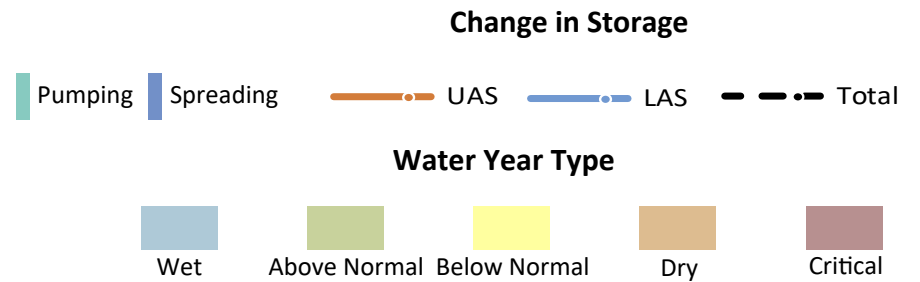
FIGURE 2-67 Water Year Type, Groundwater Use, and Annual Change in Storage in the Oxnard Subbasin Oxnard Subbasin Groundwater Sustainability Plan 2020 Annual Report
