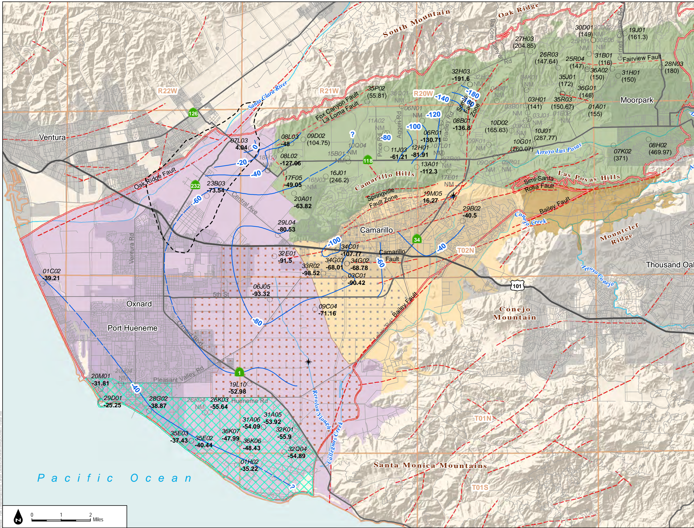
FIGURE 2-24 Groundwater Elevation Contours in the Fox Canyon Aquifer, March 2-29, 2017
