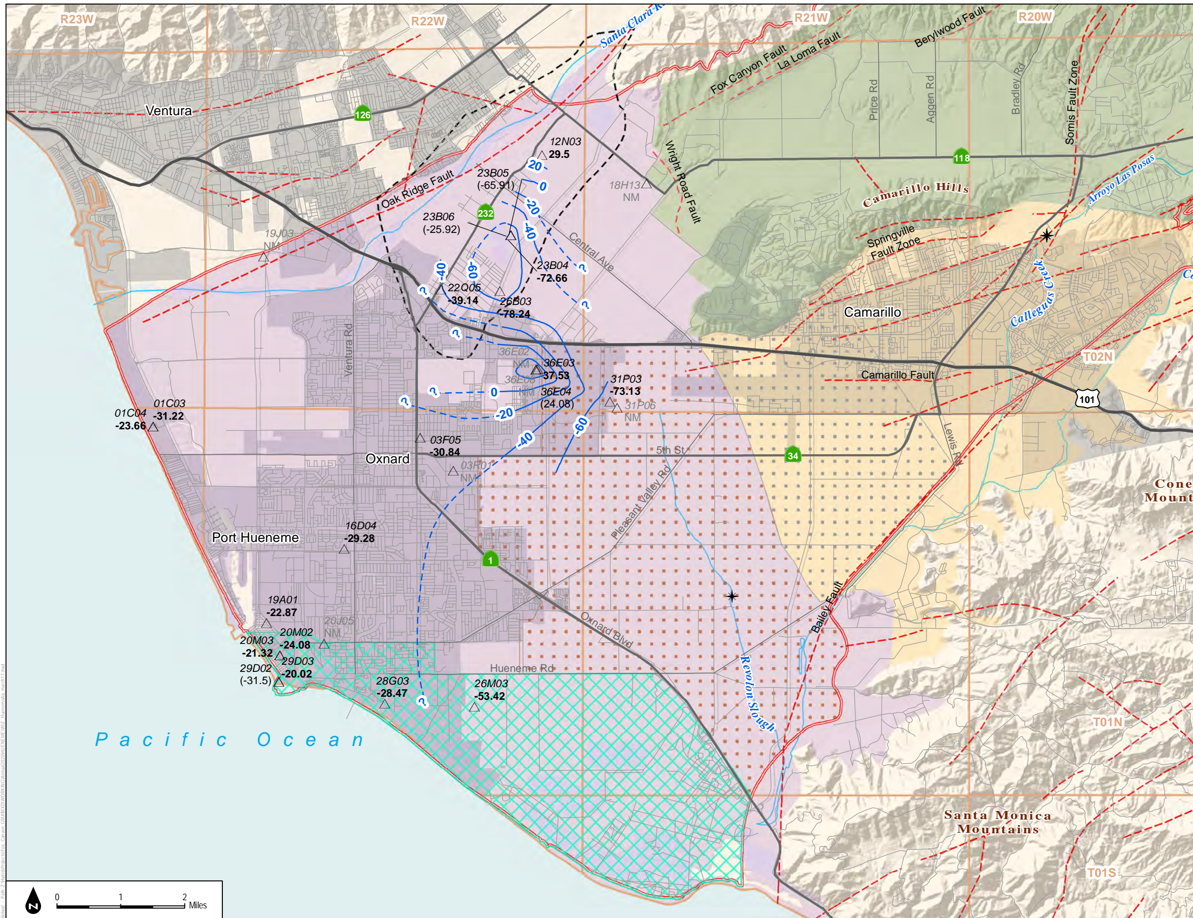
FIGURE 2-17 Groundwater Elevation Contours in the Hueneme Aquifer, March 2-29, 2017
