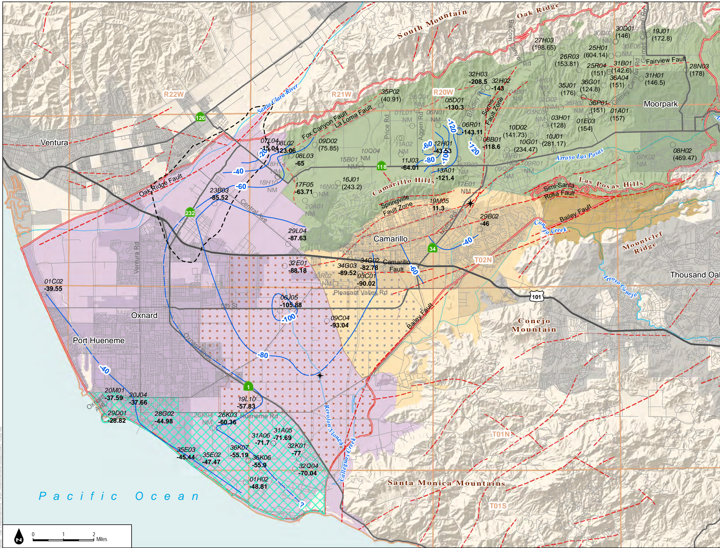
FIGURE 2-26 Groundwater Elevation Contours in the Fox Canyon Aquifer, March 2-29, 2018
