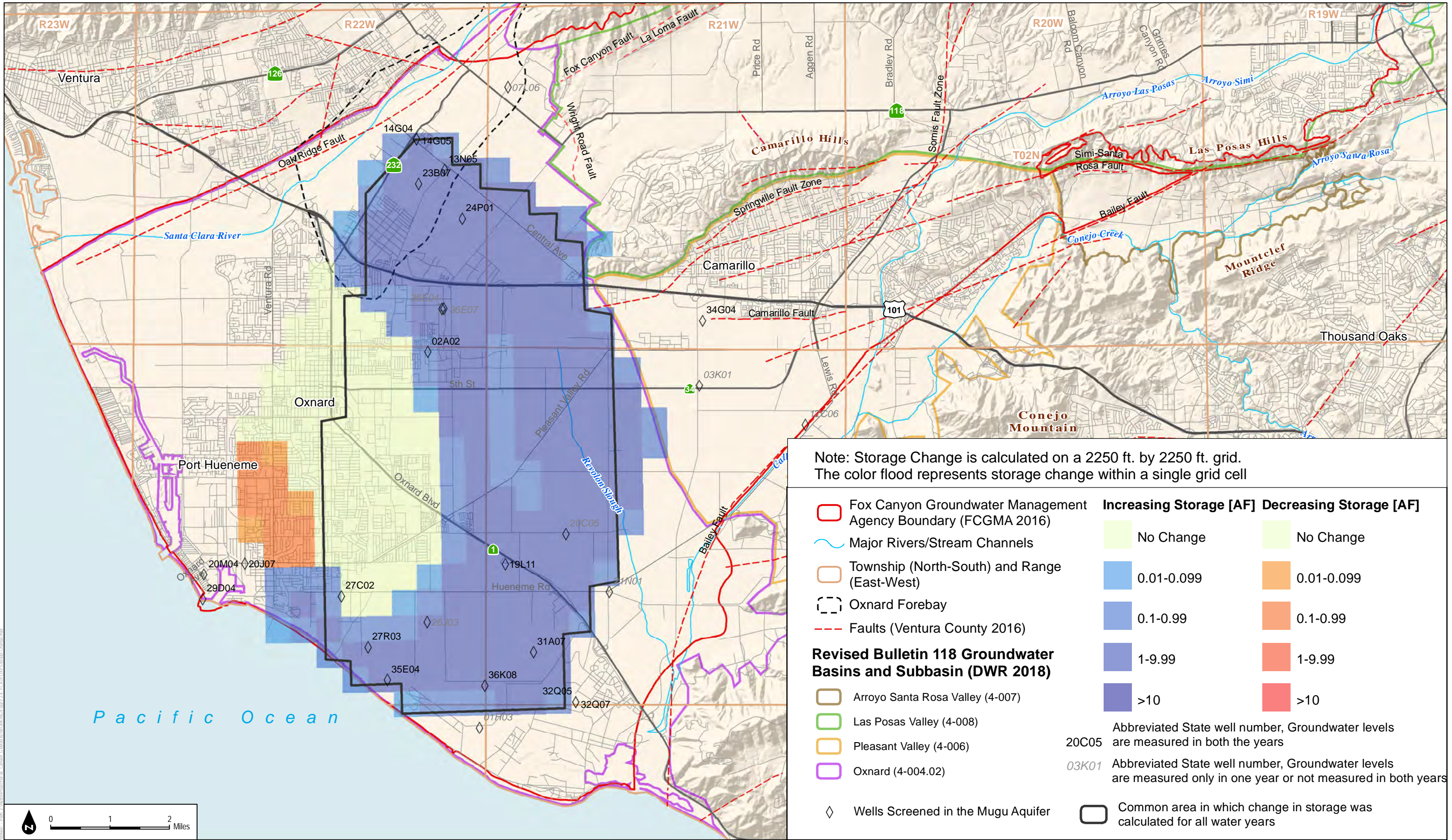
FIGURE 2-54 Change in Storage in the Mugu Aquifer: Spring 2018 to Spring 2019
