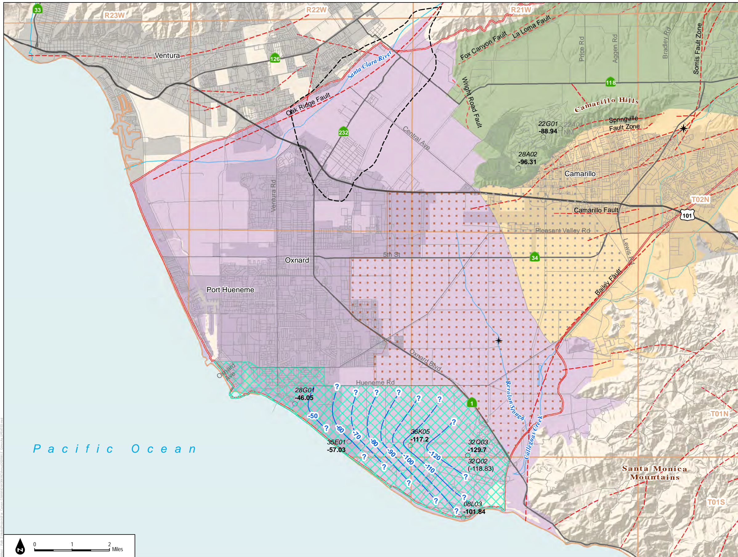
FIGURE 2-30 Groundwater Elevation Contours in the Grimes Canyon Aquifer, October 2-29, 2016
