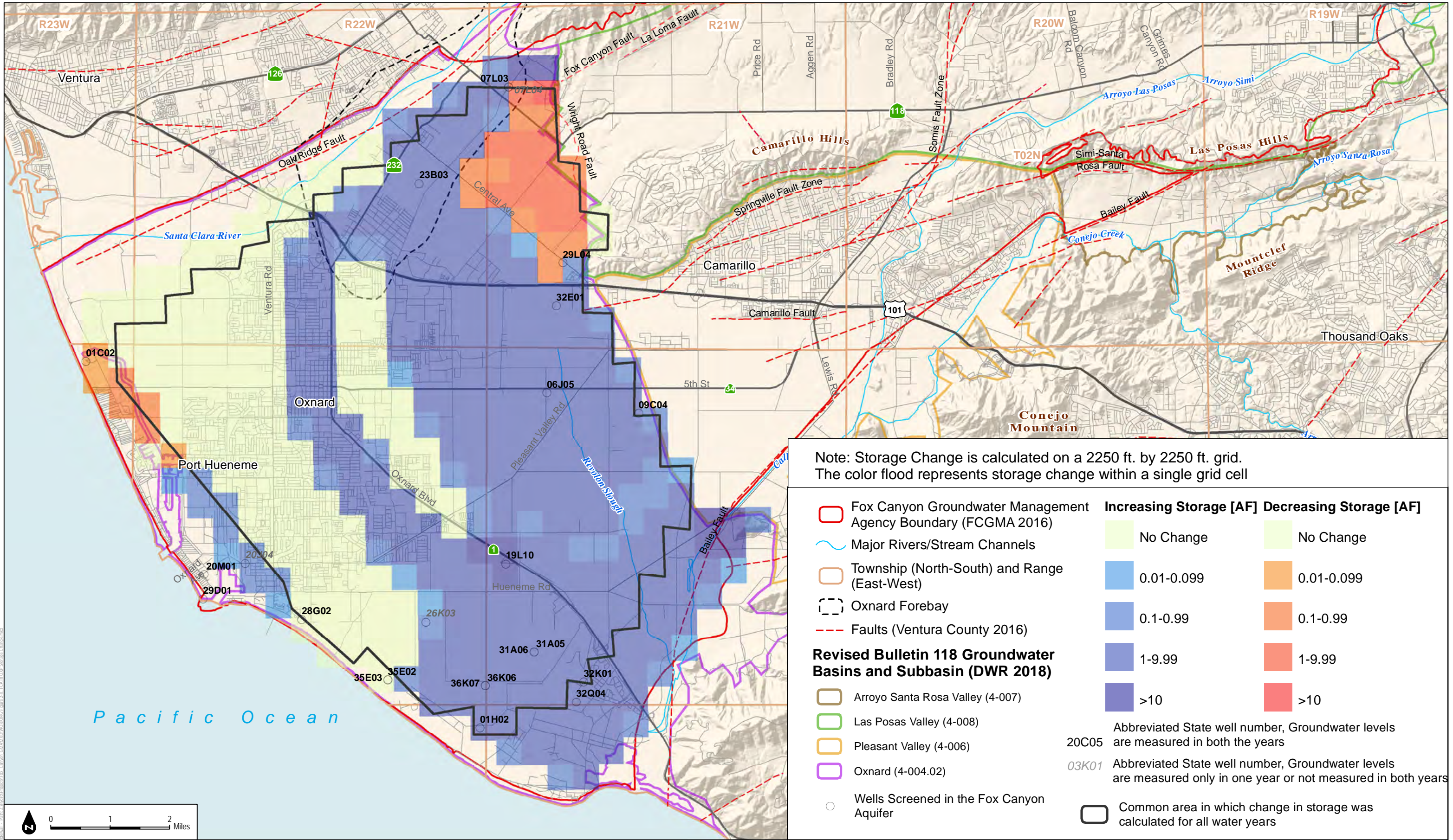
FIGURE 2-60 Change in Storage in the Fox Canyon Aquifer: Spring 2016 to Spring 2017
