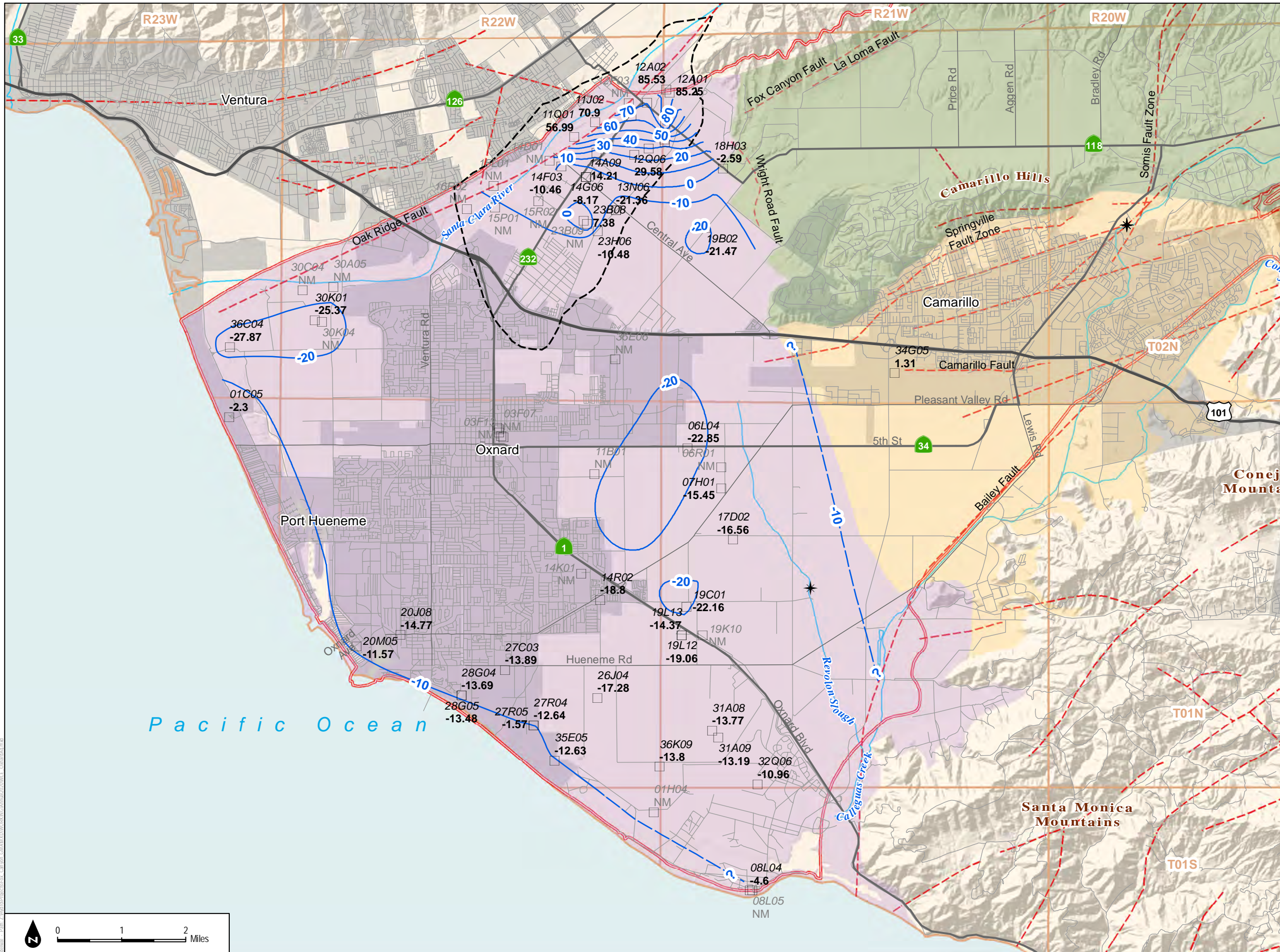
FIGURE 2-7 Groundwater Elevation Contours in the Oxnard Aquifer, March 2-29, 2019
