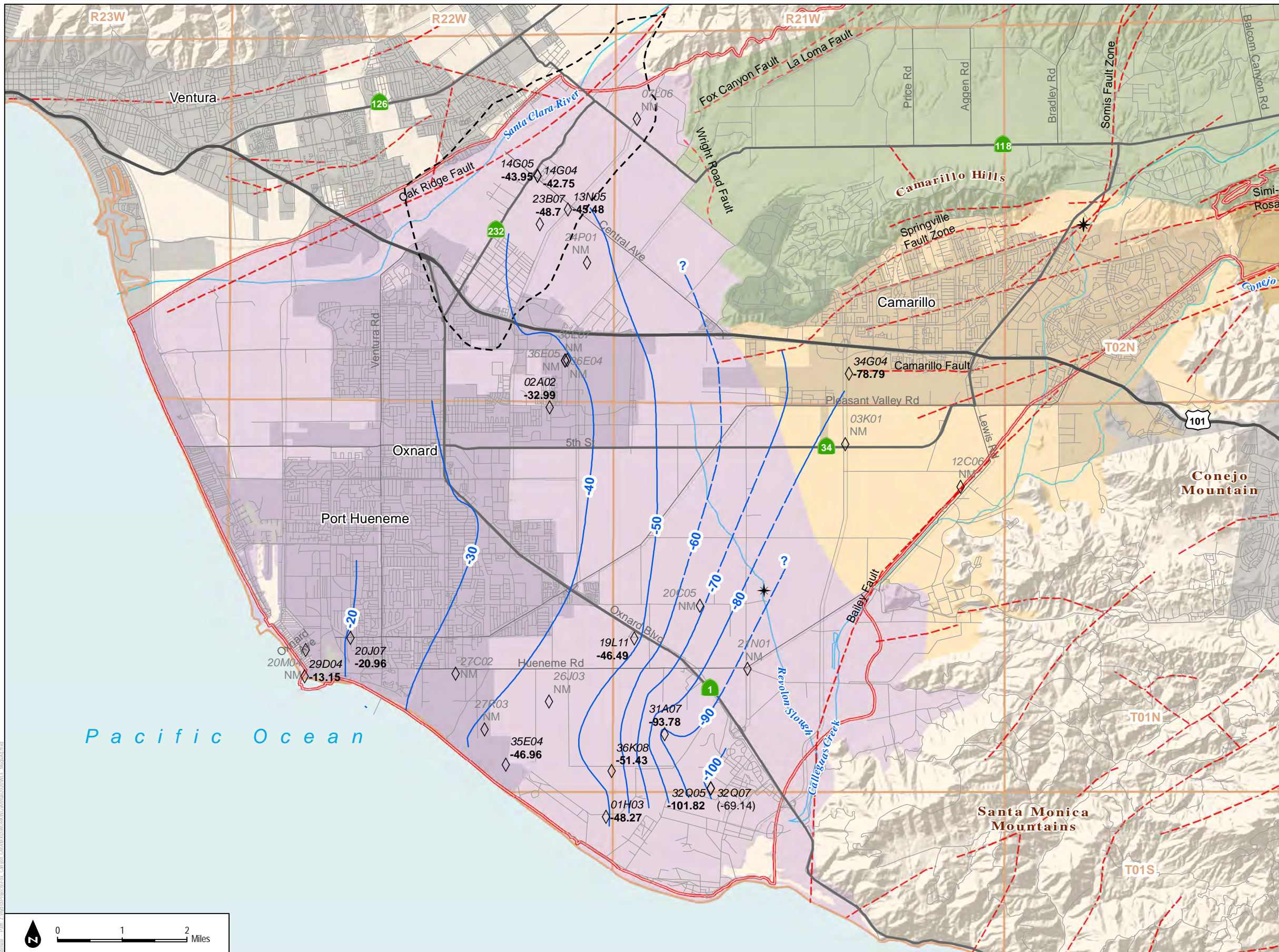
FIGURE 2-13 Groundwater Elevation Contours in the Mugu Aquifer, October 2-29, 2018
