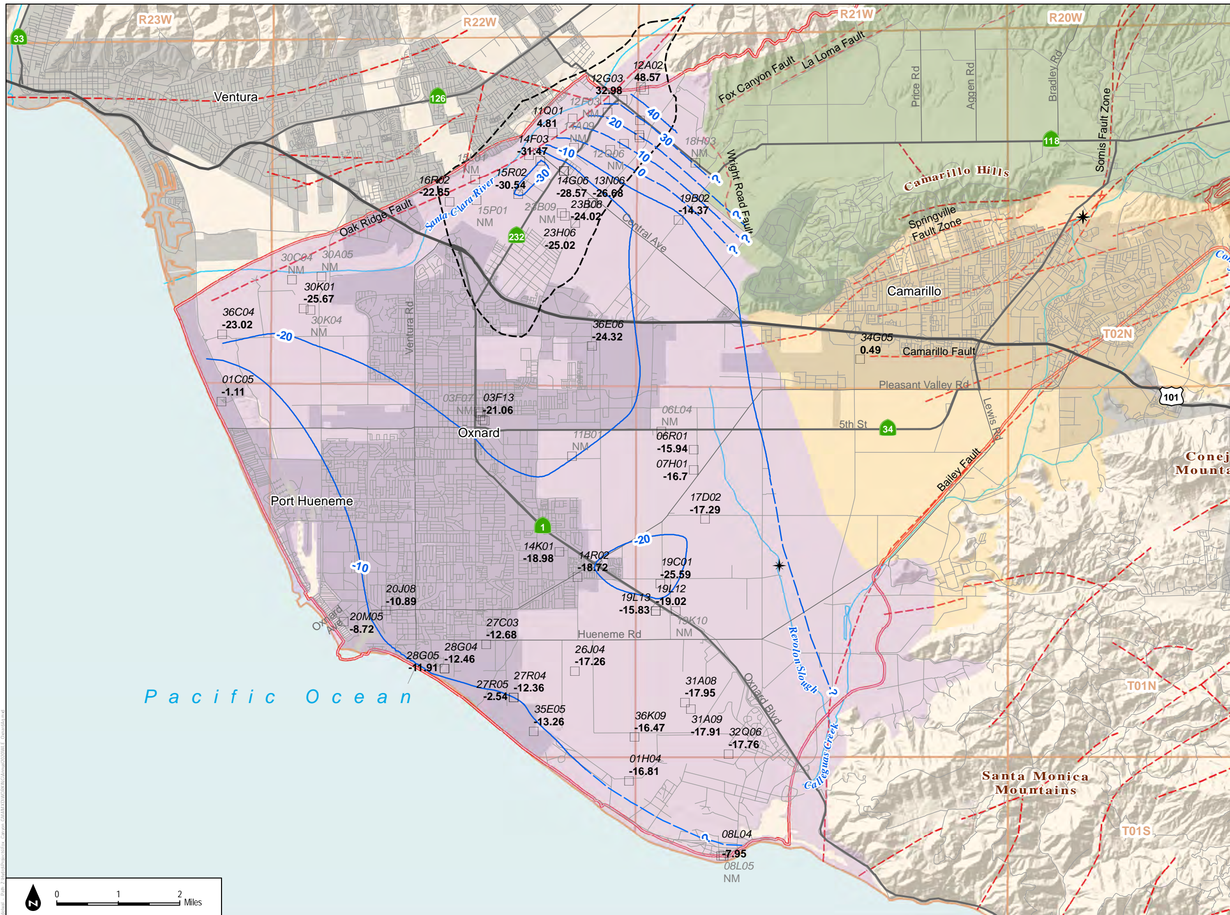
FIGURE 2-1 Groundwater Elevation Contours in the Oxnard Aquifer, March 2-29, 2016
