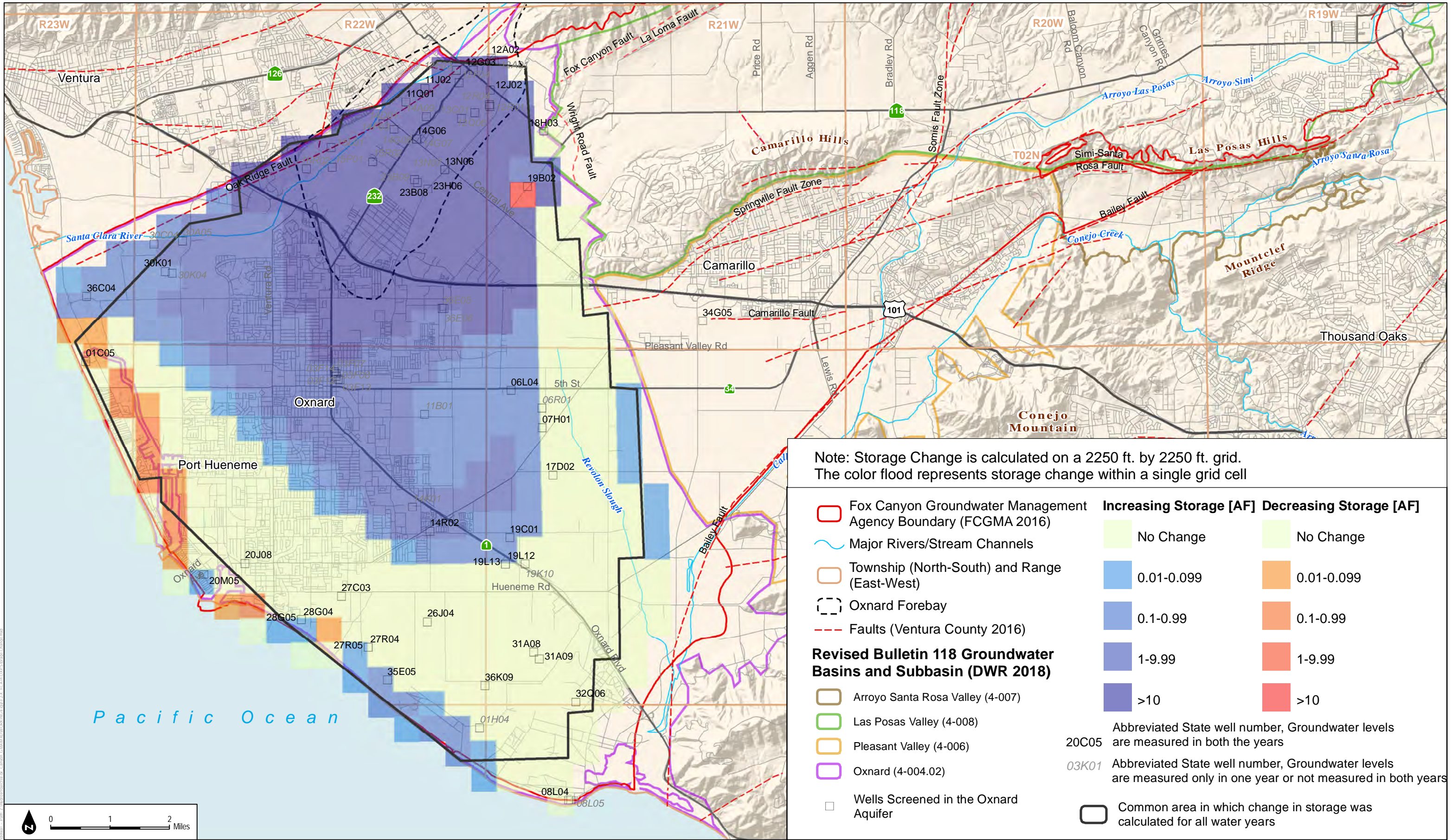
FIGURE 2-50 Change in Storage in the Oxnard Aquifer: Spring 2018 to Spring 2019
