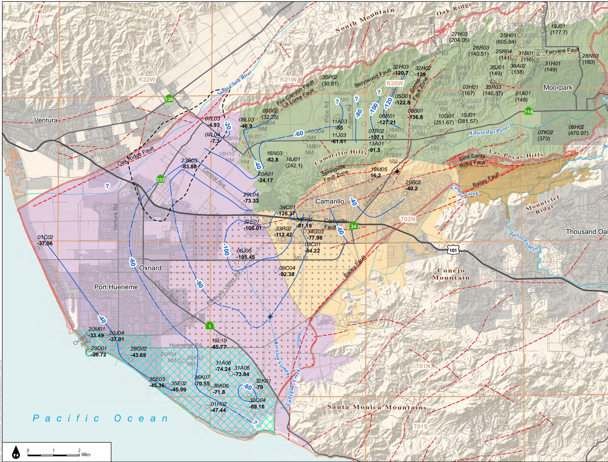
FIGURE 2-22 Groundwater Elevation Contours in the Fox Canyon Aquifer, March 2-29, 2016
