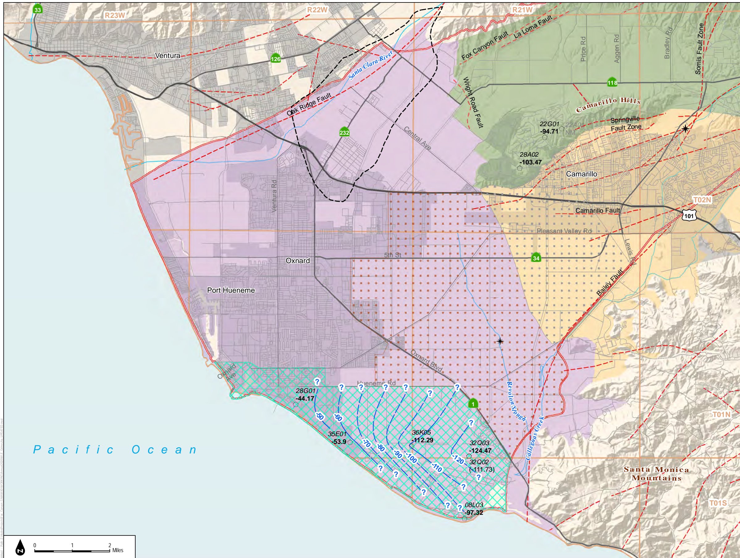
FIGURE 2-32 Groundwater Elevation Contours in the Grimes Canyon Aquifer, October 2-29, 2017
