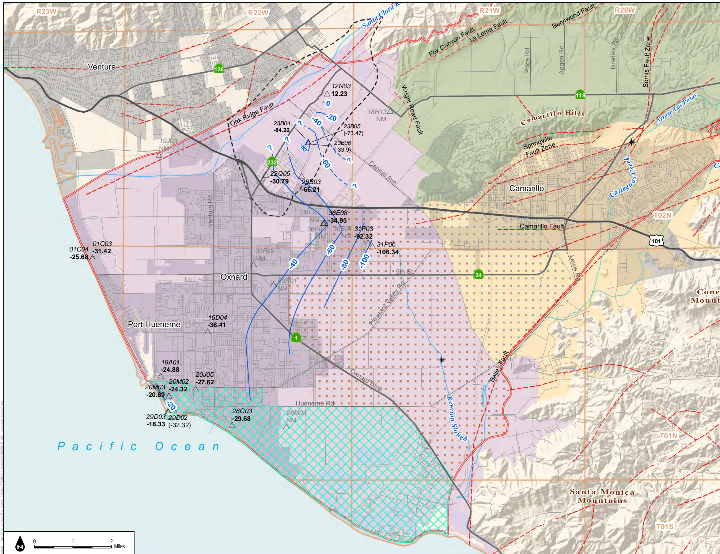
FIGURE 2-15 Groundwater Elevation Contours in the Hueneme Aquifer, March 2-29, 2016
